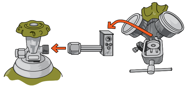
Figure - App D 5 Assembly using the adapter
