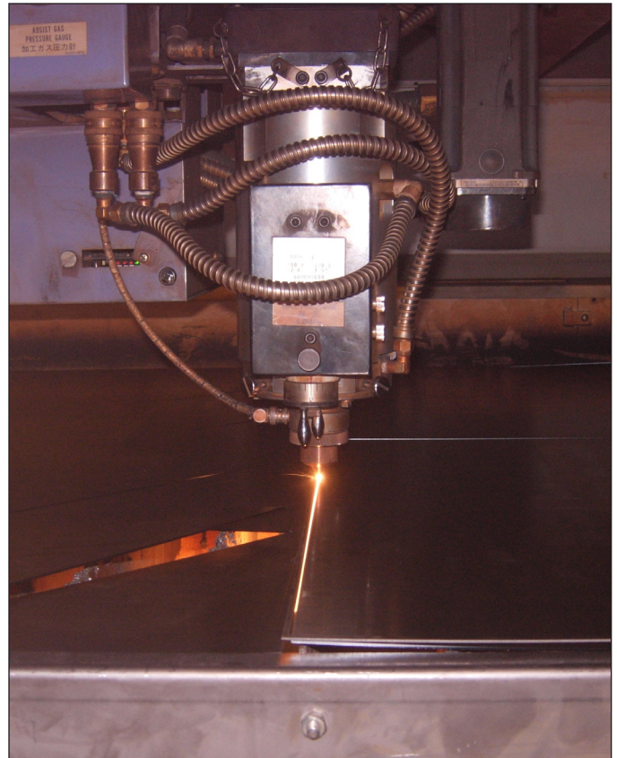
CO 2 Laser Cutting Sheet Metal
