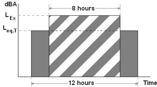
Figure 2. L eq is obtained when the noise exposure in the actual shift length (here T = 12 hours) is adjusted to the standard shift time of 8 hours
