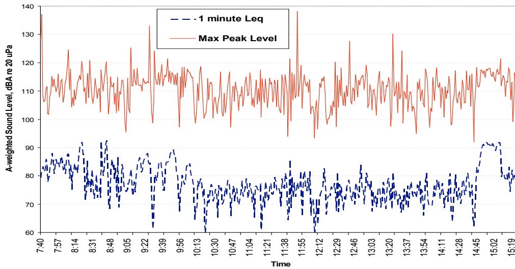
Figure 9. Data Logging Dosimeter Printout with Peak Artifacts
