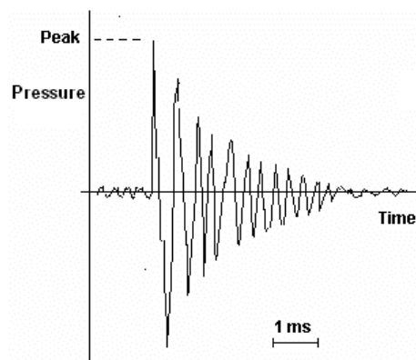
Figure 4. Time Record of an Impact Noise
