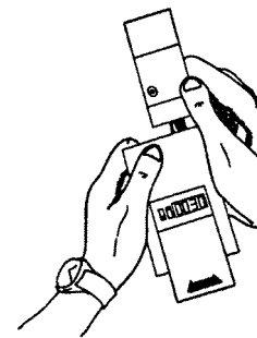
Figure 7. Calibrating a Basic Personal Noise Dosimeter
