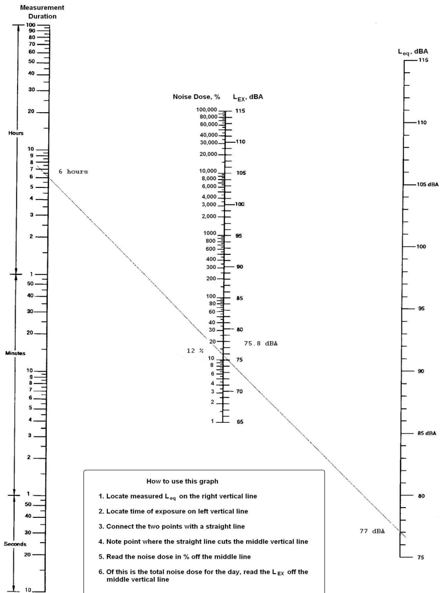
Nomograph of L_{eq} , L_{EX} , Noise Dose and Time
