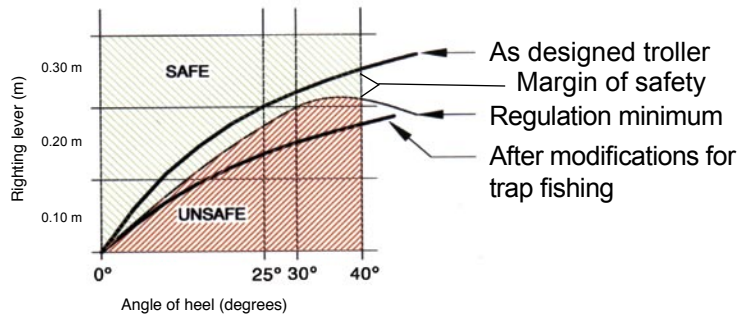
Vessel: Righting Energy Diagram
